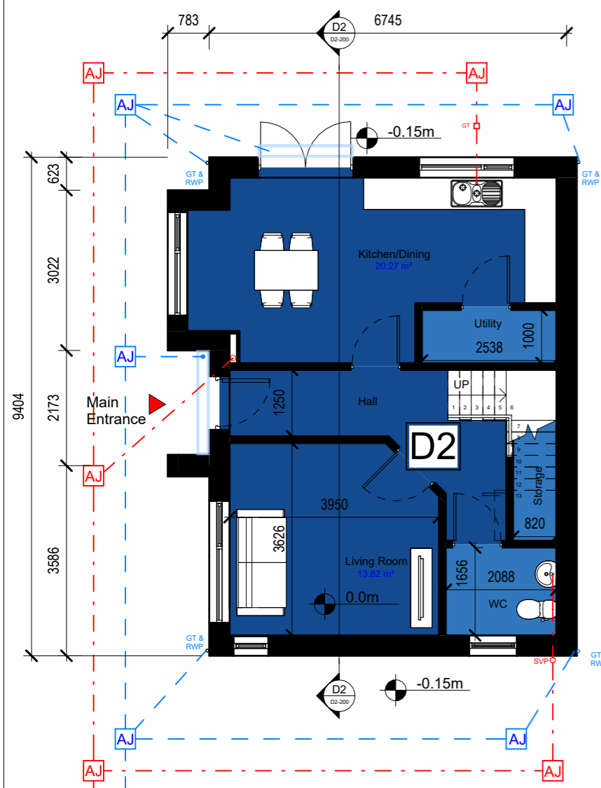
01 GROUND FLOOR PLAN 1:100@A3 7826
