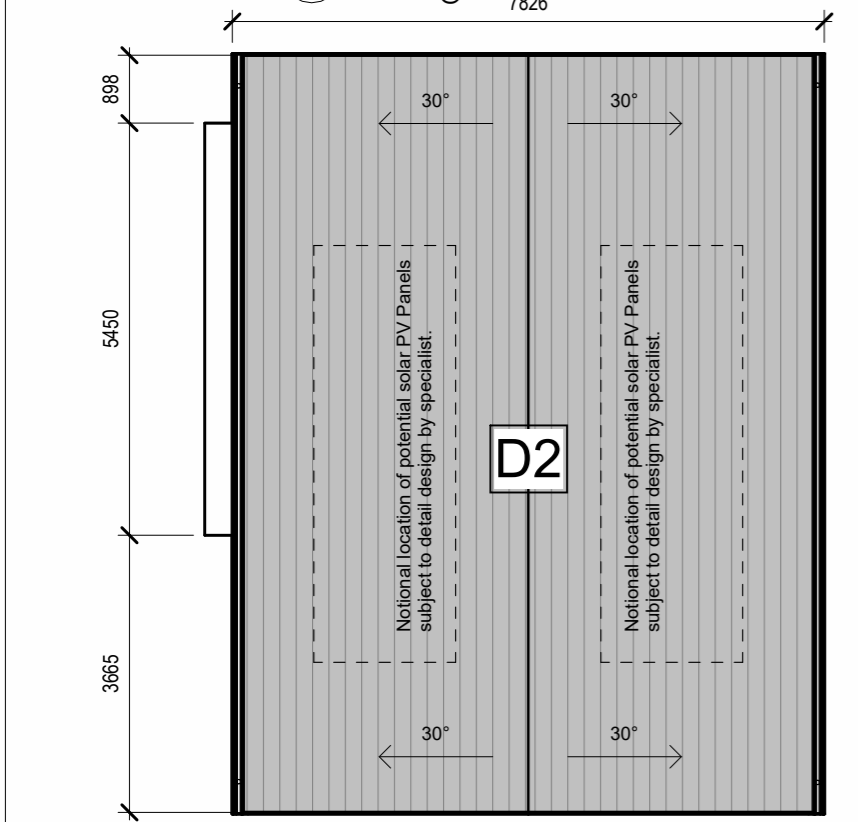
03 ROOF PLAN 1:100@A3
