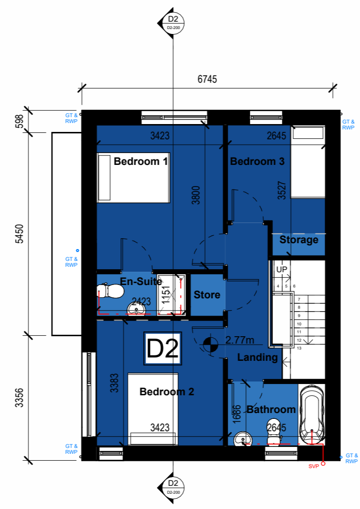
02 FIRST FLOOR PLAN 1:100@A3
